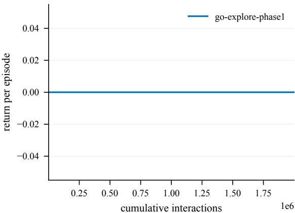
Return -- OpenFieldChamberCount10-610@1
