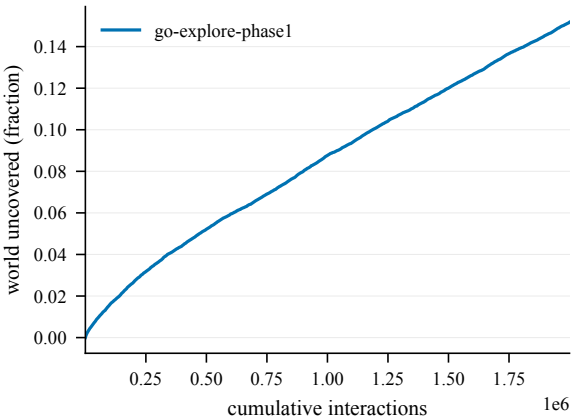
Cumulative coverage -- OpenFieldChamberCount10-610@1
