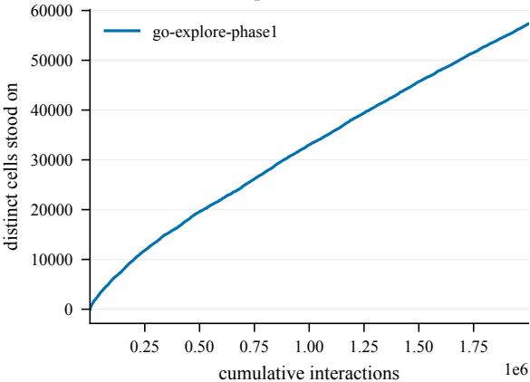
States discovered -- OpenFieldChamberCount10-610@3
