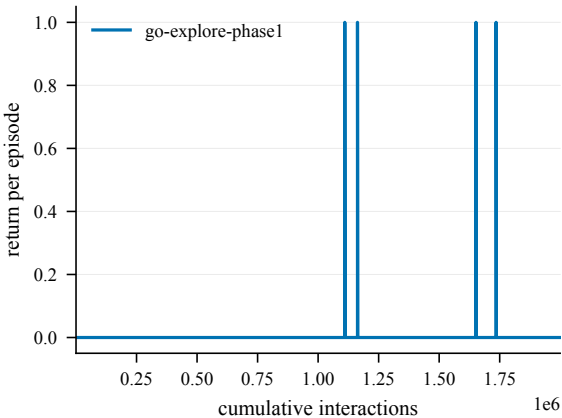
Return -- OpenFieldChamberCount4-500@2
