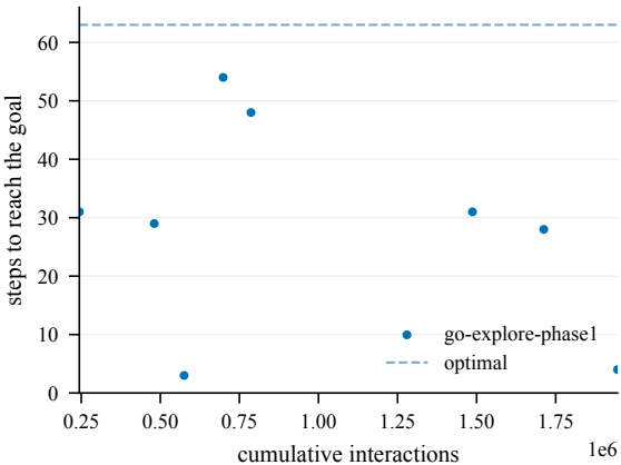
Steps to goal (train) -- OpenFieldChamberCount4-500@4
