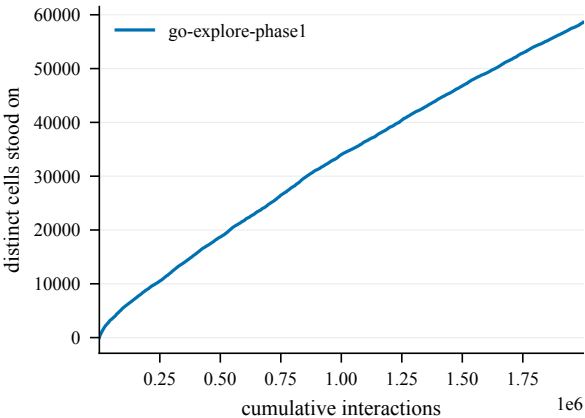
States discovered -- OpenFieldChamberCount4-500@4
