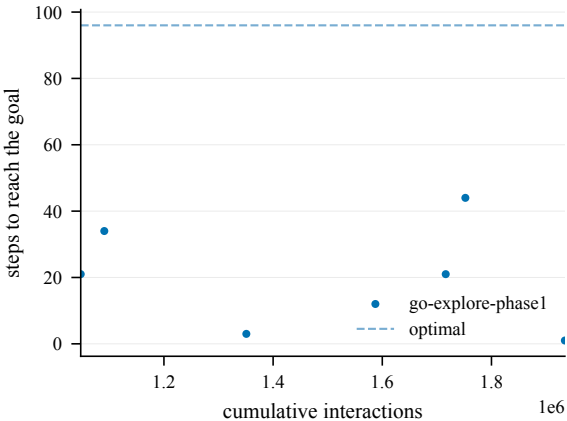
Steps to goal (train) -- OpenFieldChamberCount6-530@4
