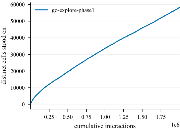
States discovered -- OpenFieldChamberCount6-530@4
