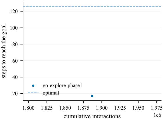
Steps to goal (train) -- OpenFieldChamberCount8-570@1
