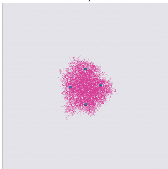
Go-Explore
