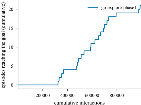
Goal reached -- Bottleneck3-100@4000
