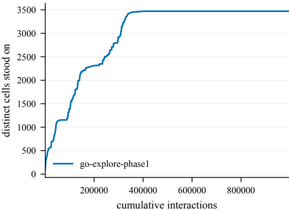
States discovered -- Bottleneck3-100@4000
