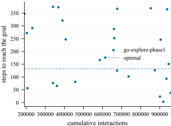
Steps to goal (train) -- Bottleneck3-100@4001
