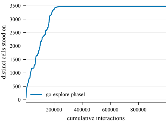
States discovered -- Bottleneck3-100@4001
