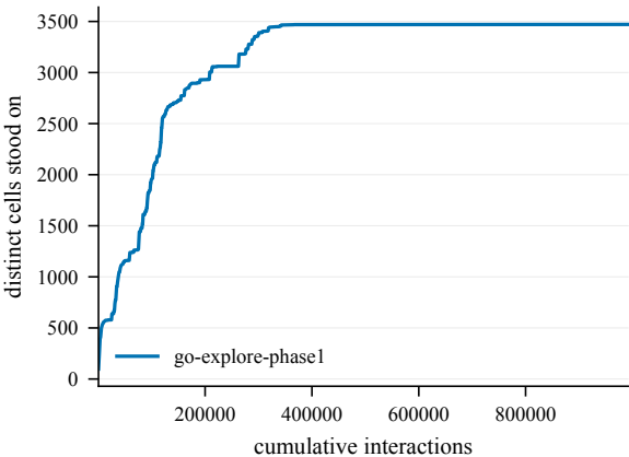
States discovered -- Bottleneck3-100@4002
