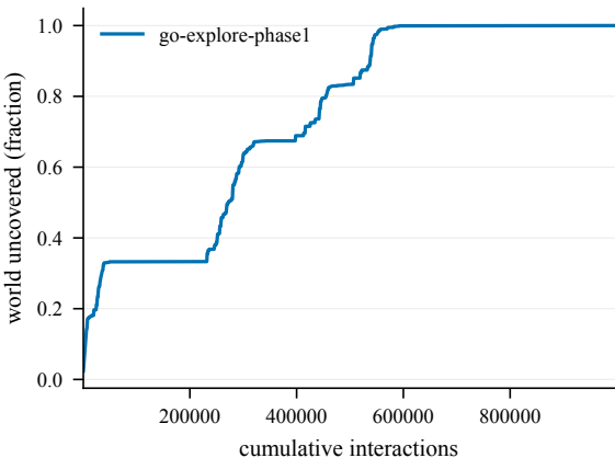
Cumulative coverage -- Bottleneck3-200@4000
