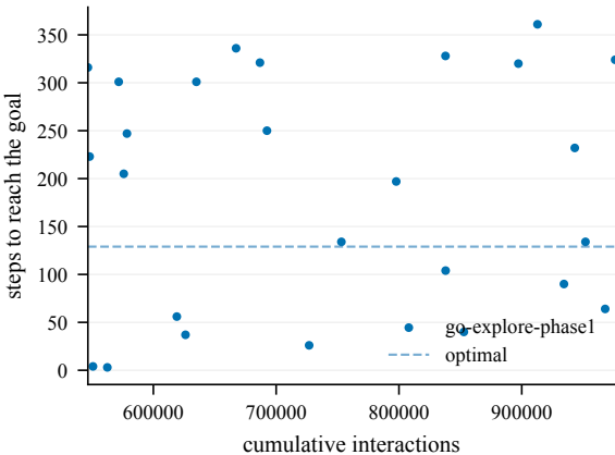
Steps to goal (train) -- Bottleneck3-200@4000
