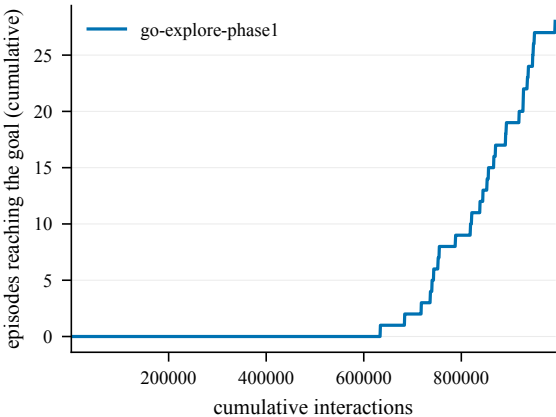
Goal reached -- Bottleneck3-200@4001
