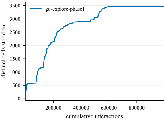
States discovered -- Bottleneck3-200@4001
