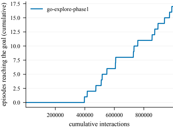
Goal reached -- Bottleneck6-100@4000
