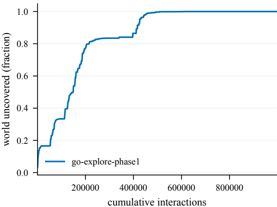
Cumulative coverage -- Bottleneck6-100@4000
