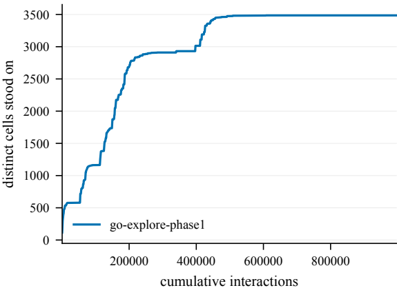
States discovered -- Bottleneck6-100@4000
