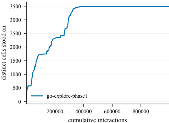
States discovered -- Bottleneck6-100@4001
