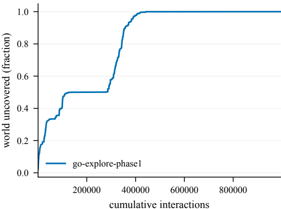
Cumulative coverage -- Bottleneck6-100@4002
