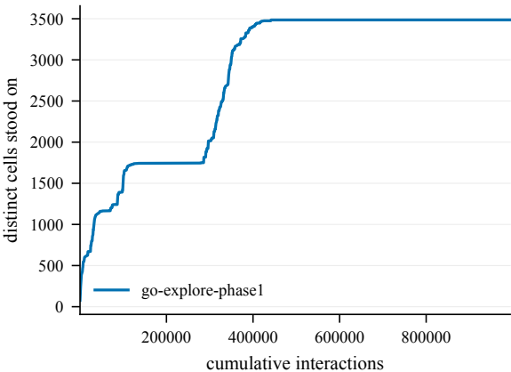
States discovered -- Bottleneck6-100@4002
