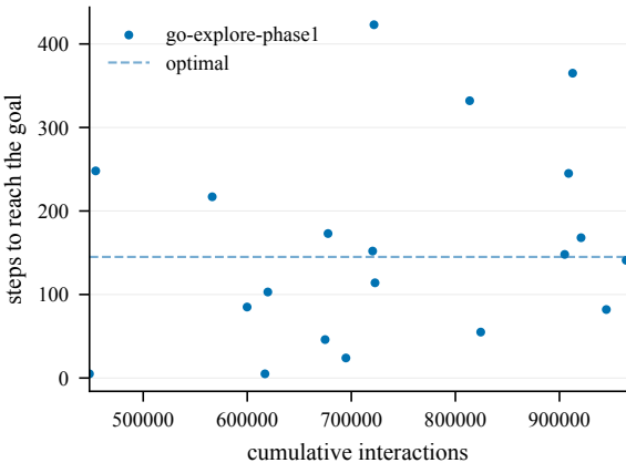
Steps to goal (train) -- Bottleneck6-200@4000
