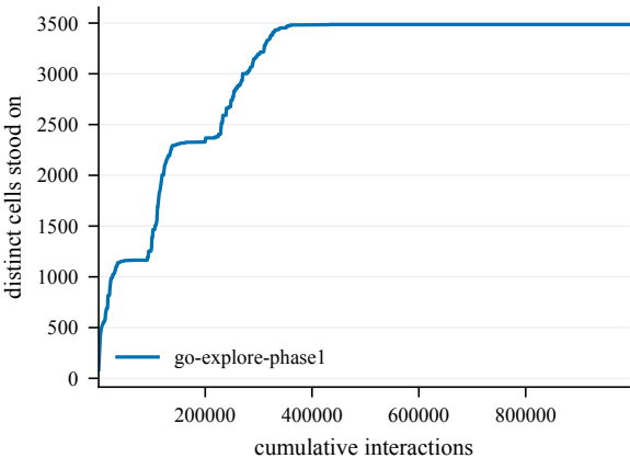
States discovered -- Bottleneck6-200@4001
