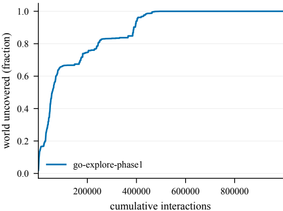
Cumulative coverage -- Bottleneck6-200@4002
