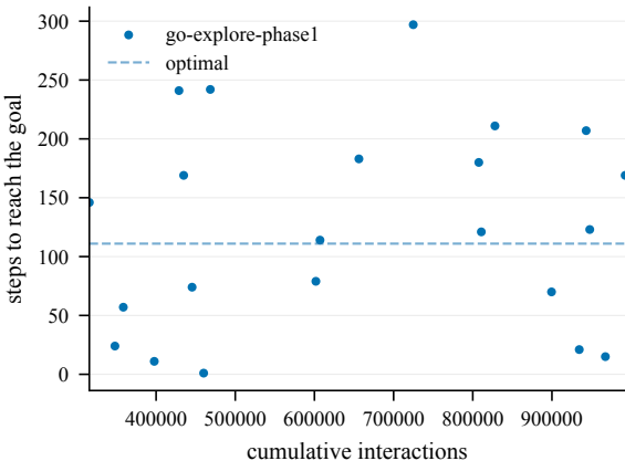
Steps to goal (train) -- Bottleneck6-200@4002
