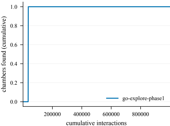
Chambers -- ChamberCount1-100@4000
