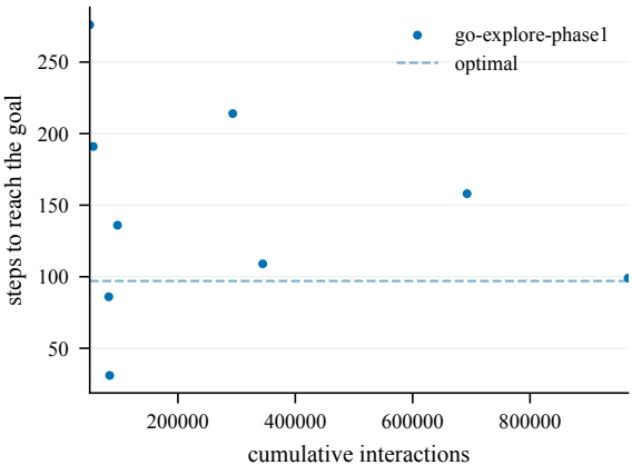
Steps to goal (train) -- ChamberCount1-100@4000
