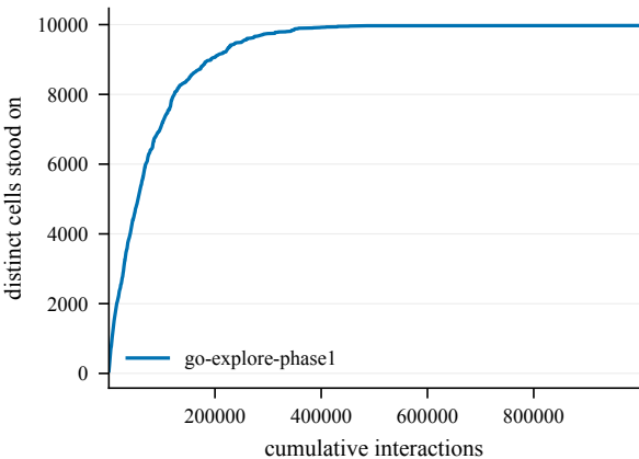
States discovered -- ChamberCount1-100@4000
