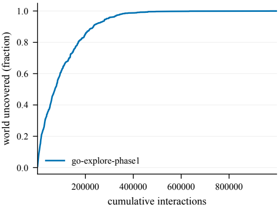
Cumulative coverage -- ChamberCount1-100@4001
