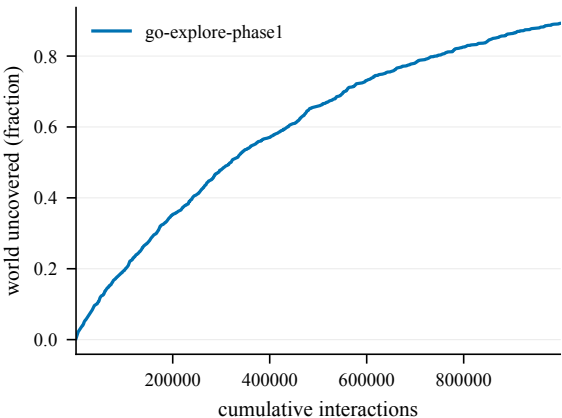
Cumulative coverage -- ChamberCount1-200@4001
