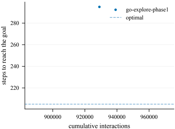
Steps to goal (train) -- ChamberCount1-200@4001
