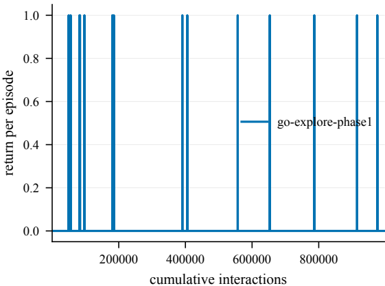
Return -- ChamberCount2-100@4000
