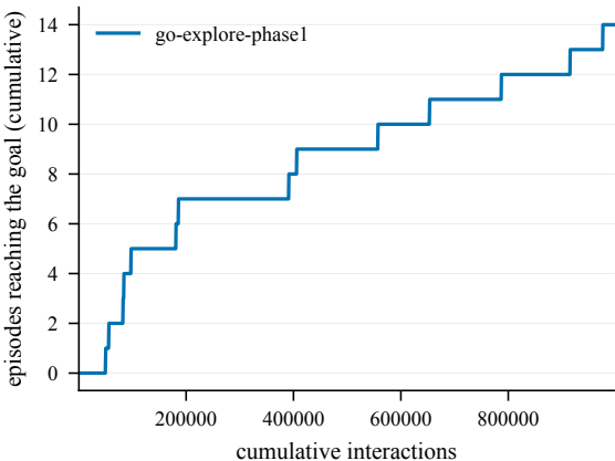
Goal reached -- ChamberCount2-100@4000
