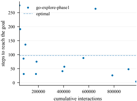
Steps to goal (train) -- ChamberCount2-100@4000
