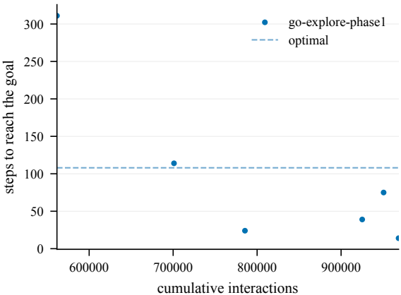
Steps to goal (train) -- ChamberCount2-100@4001
