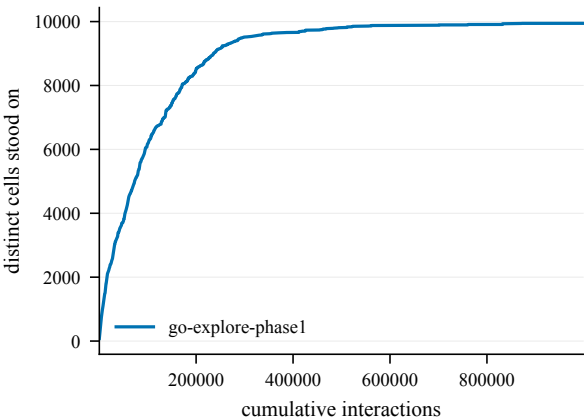
States discovered -- ChamberCount2-100@4001
