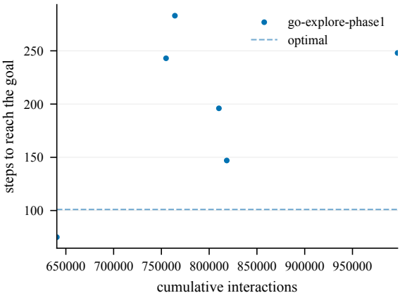
Steps to goal (train) -- ChamberCount2-100@4002
