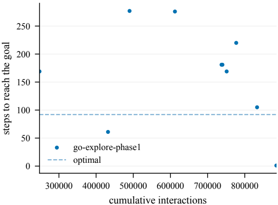
Steps to goal (train) -- ChamberCount4-100@4000
