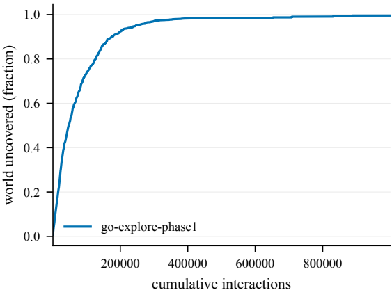
Cumulative coverage -- ChamberCount4-100@4001
