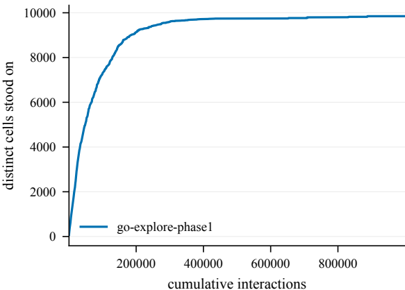
States discovered -- ChamberCount4-100@4001
