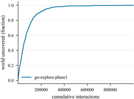
Cumulative coverage -- ChamberCount4-100@4002
