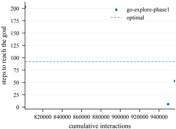
Steps to goal (train) -- ChamberCount4-100@4002
