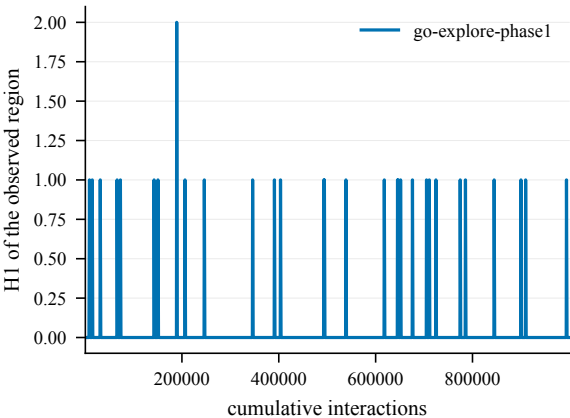
Discovered topology -- ChamberCount4-200@4000
