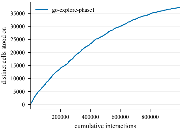
States discovered -- ChamberCount4-200@4002
