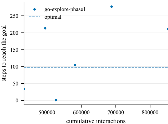
Steps to goal (train) -- ChamberCount8-100@4000
