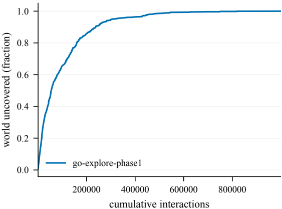
Cumulative coverage -- ChamberCount8-100@4001
